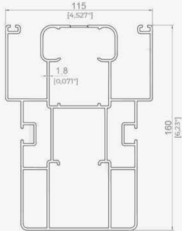
EKO RAY PROFİLİ / ECO RAIL PROFILE
