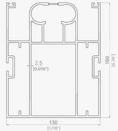
RAY PROFİLİ / RAIL PROFILE
