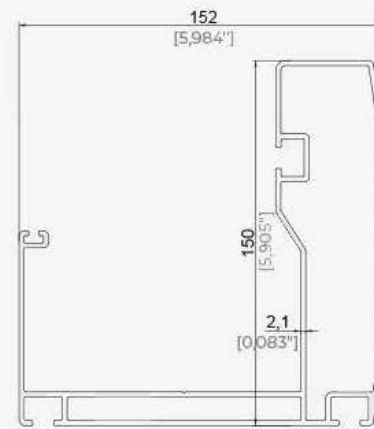
152x150 Dere Profili 152x150 Gutter Profile
